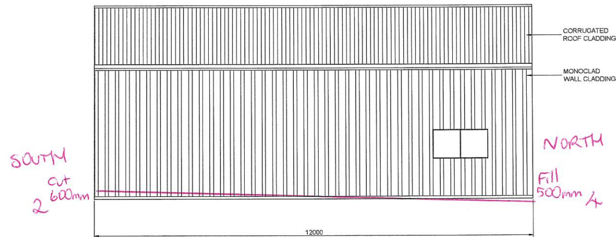
1 SIDEWALL EXTERIOR ELEVATION SCALE: 1 = 100
