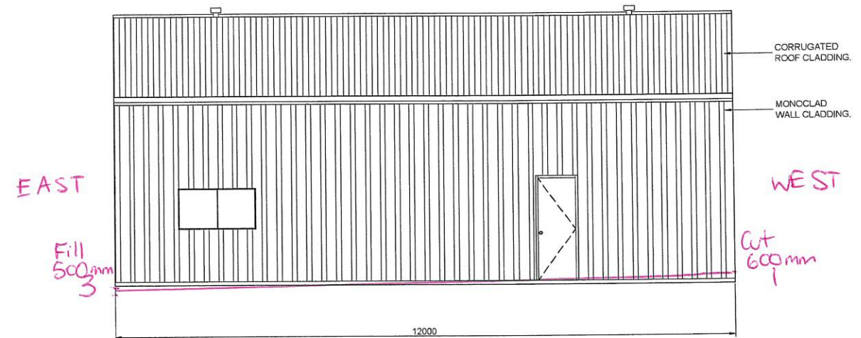
2 SIDEWALL EXTERIOR ELEVATION SCALE: 1 = 100
